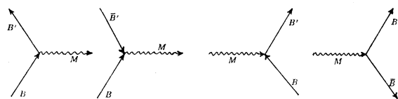
FIG. 1. Diagrams for elementary strong interactions.
